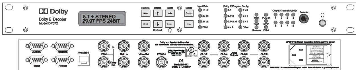
Figure 2-9 Front and Back Panels of the DP572
