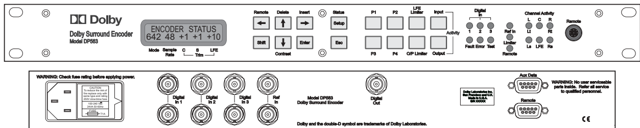
Figure 2-3 Front and Back Panels of the DP563
