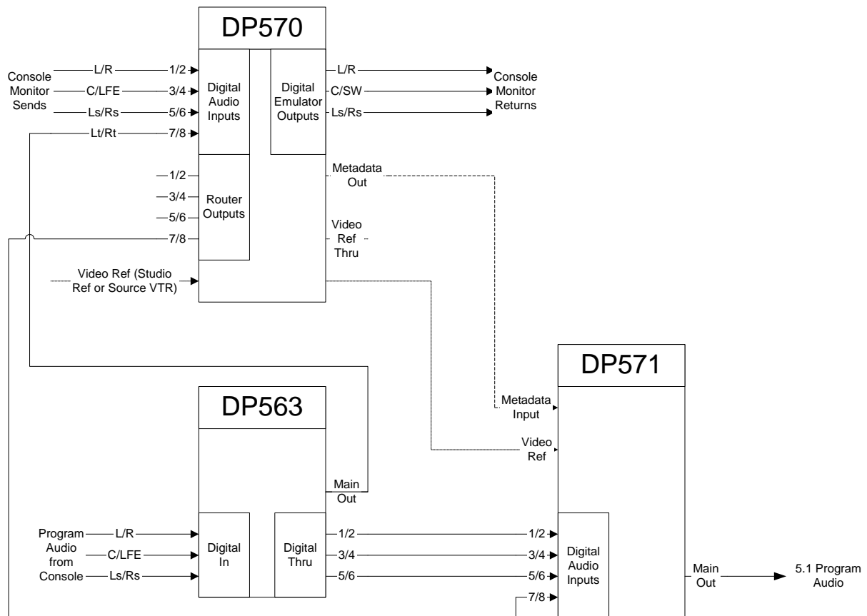
Figure 5-3 Example Equipment Setup for use with Consoles with Full Monitoring Functions
