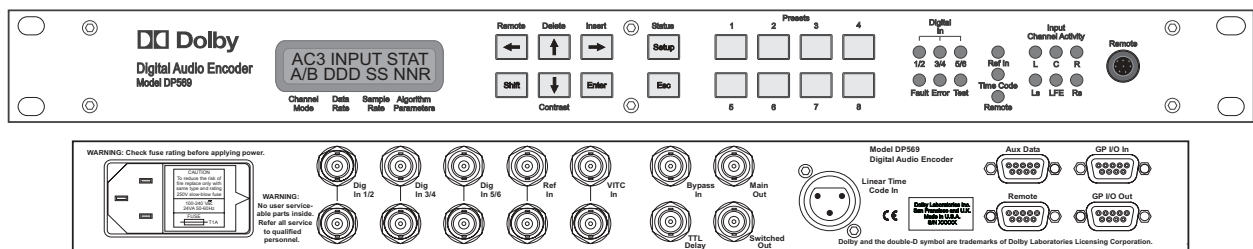
Figure 2-6 Front and Back Panels of the DP569
