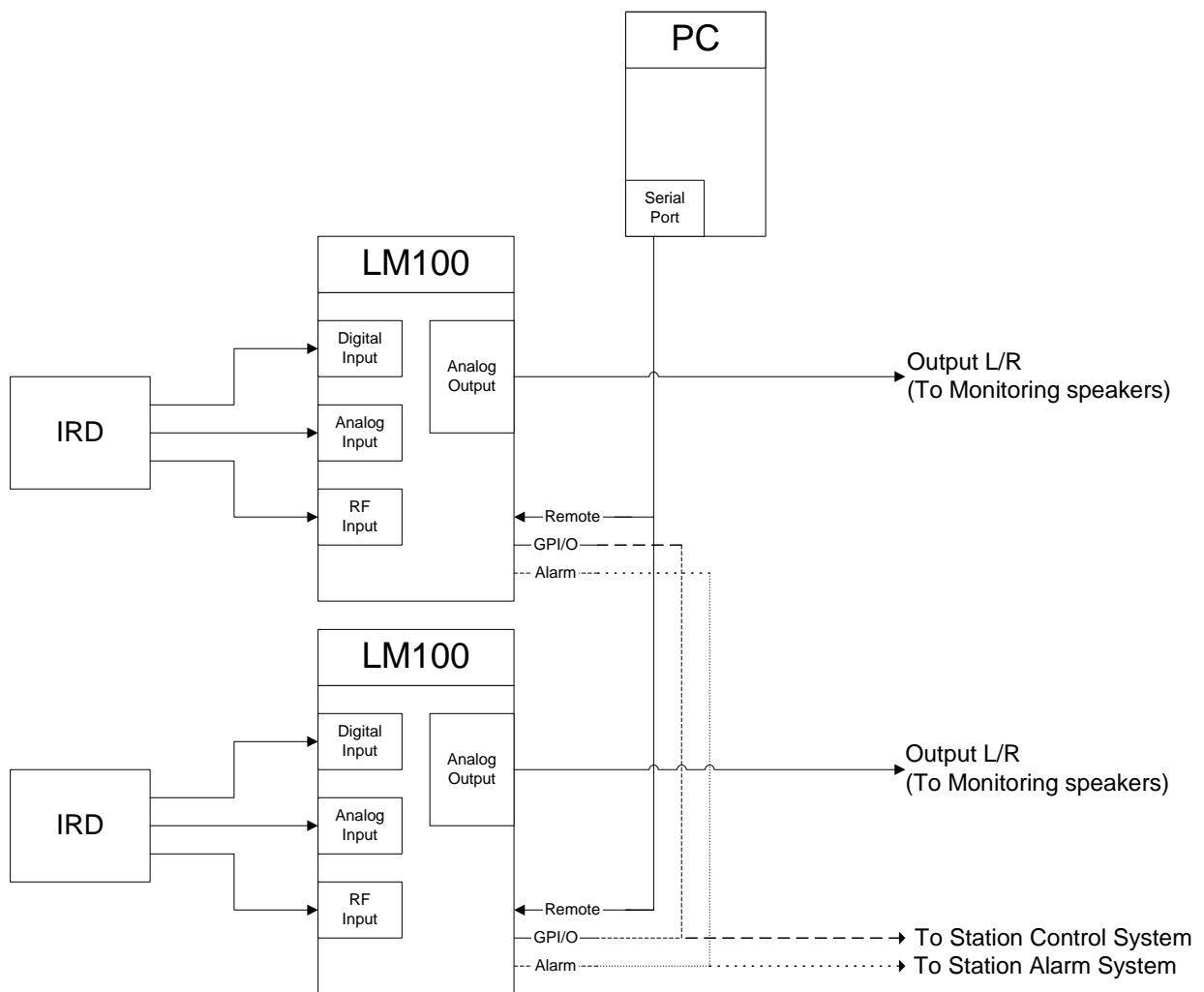
Figure 5-6 LM100 for Off-Air Analog Monitoring
