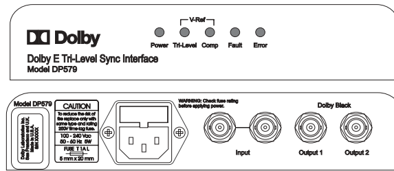
Figure 2-11 Front and Back Panels of the DP579
