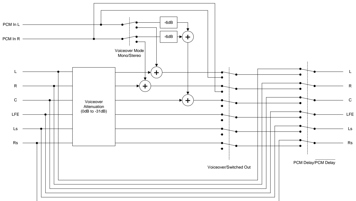
Figure 2-10 Diagram of Voiceover and Switched Output Operation
