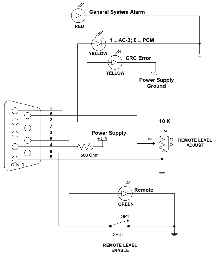
Figure 2-2 Test Box Schematic
