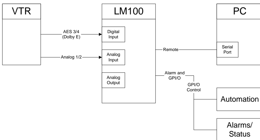
Figure 5-5 LM100 for Ingest Monitoring
