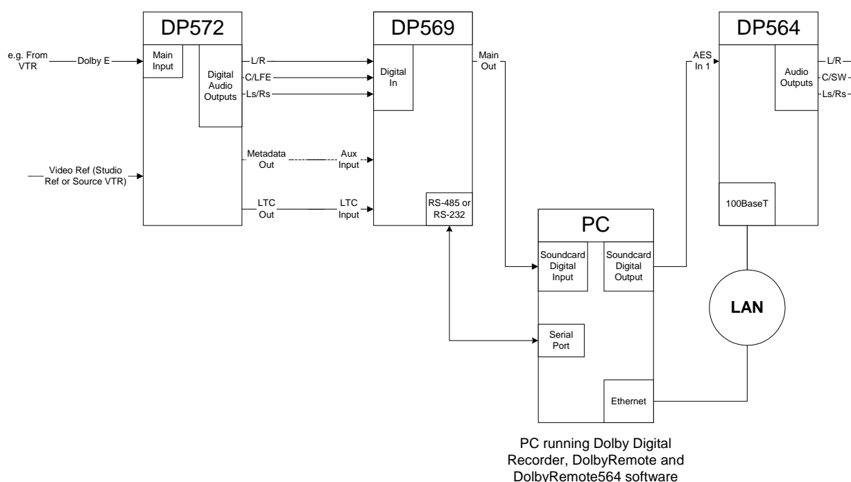
Figure 5-1 Typical DVD Encoding System
