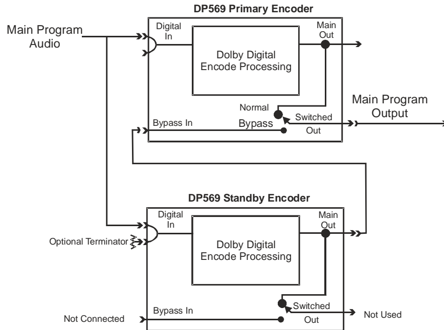
Figure 4-1 Hot Standby Operation of the DP569
