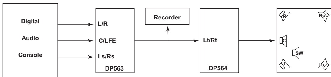
Figure A-1 Audio Flow for Surround Mixing
