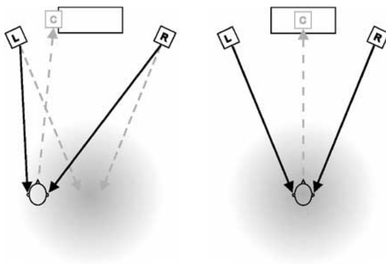
Figure A-4 Phantom Center Images with Listener Off-Center (Left) and in Sweet Spot (Right)
