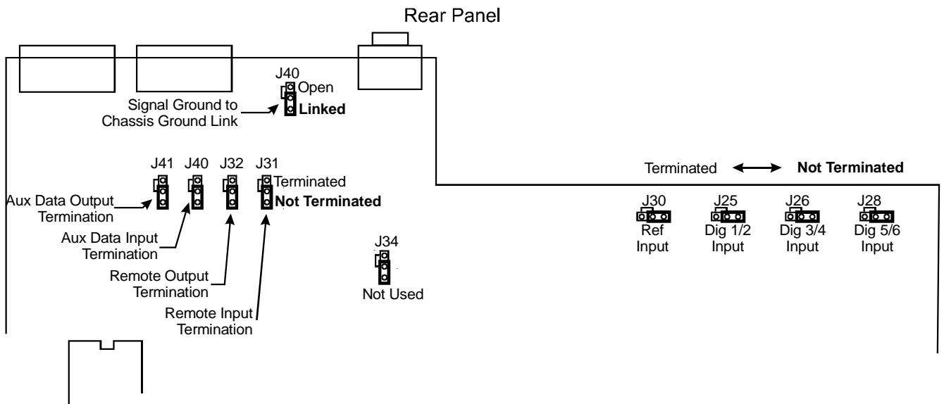
Figure 2-1 Jumper Locations
