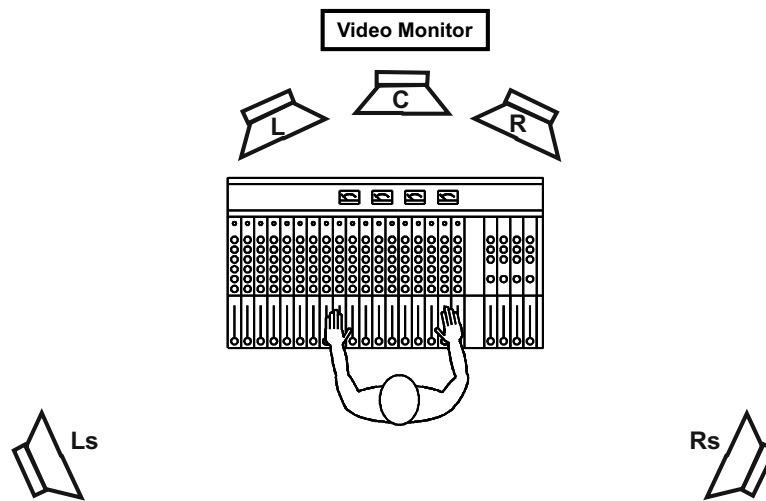
Figure A-2 Speaker Placement: Top View
