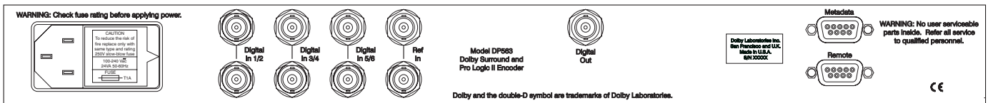
Figure 6–1 DP563 Rear Panel
