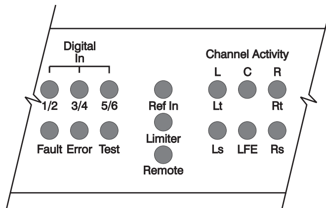
Figure 2-4 Front-Panel Indicators
