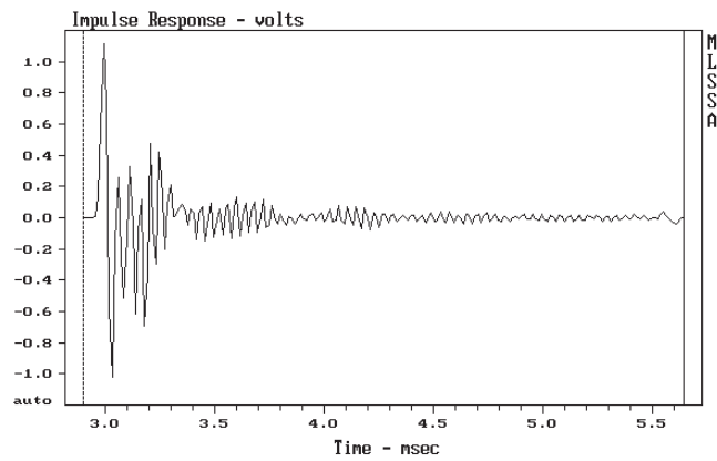
Conventional 2" Compression Driver
