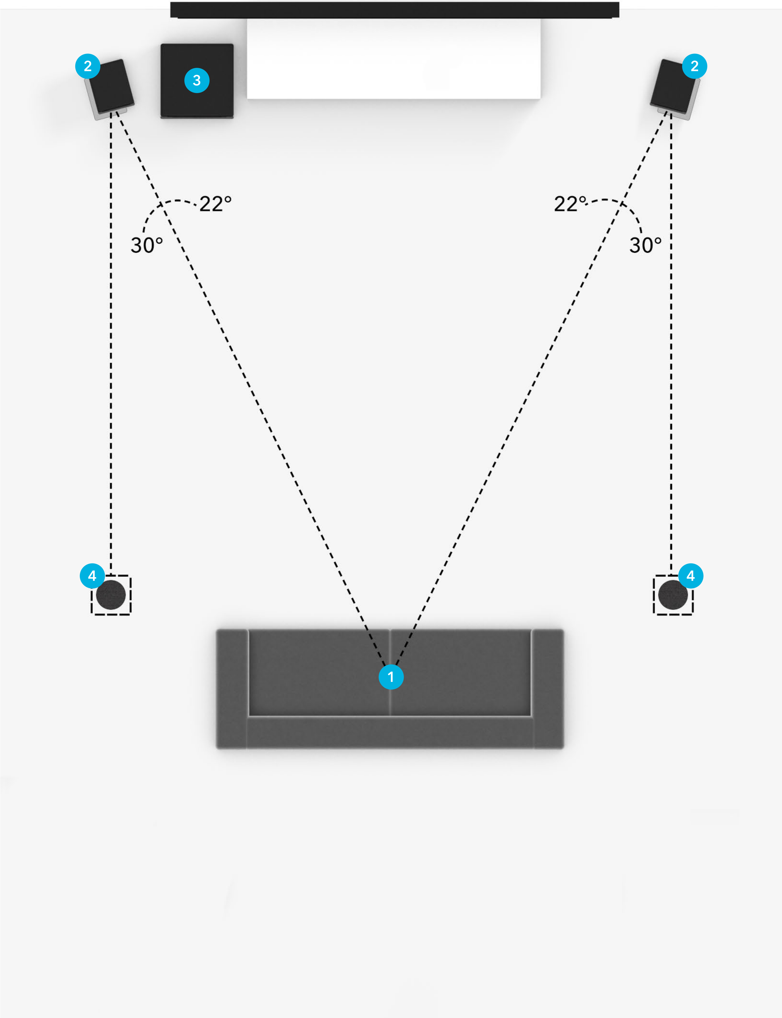
SPEAKER PLACEMENT FOR 2.1.2 SETUP
