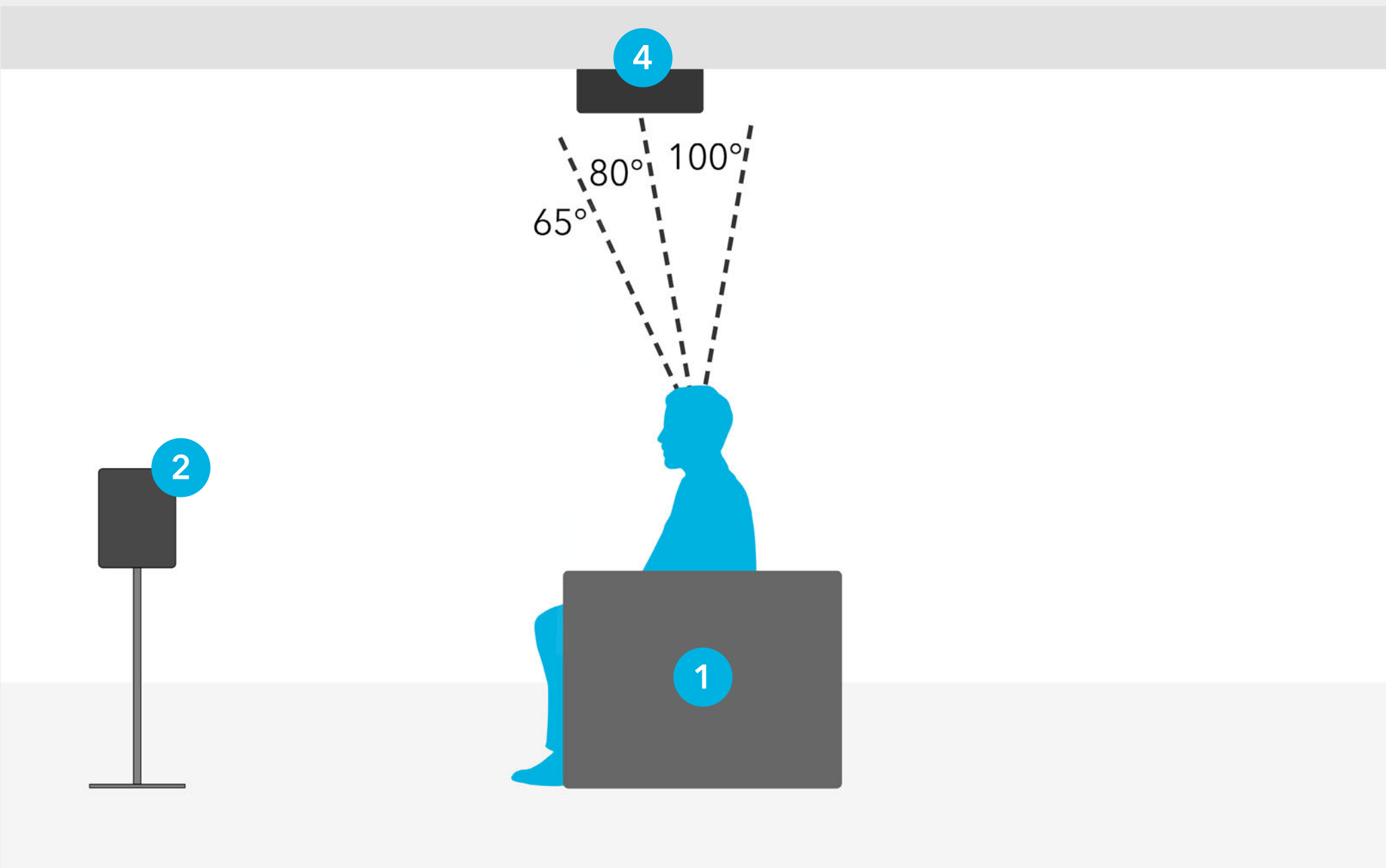
OVERHEAD SPEAKER PLACEMENT DETAIL FOR 2.1.2 SETUP
