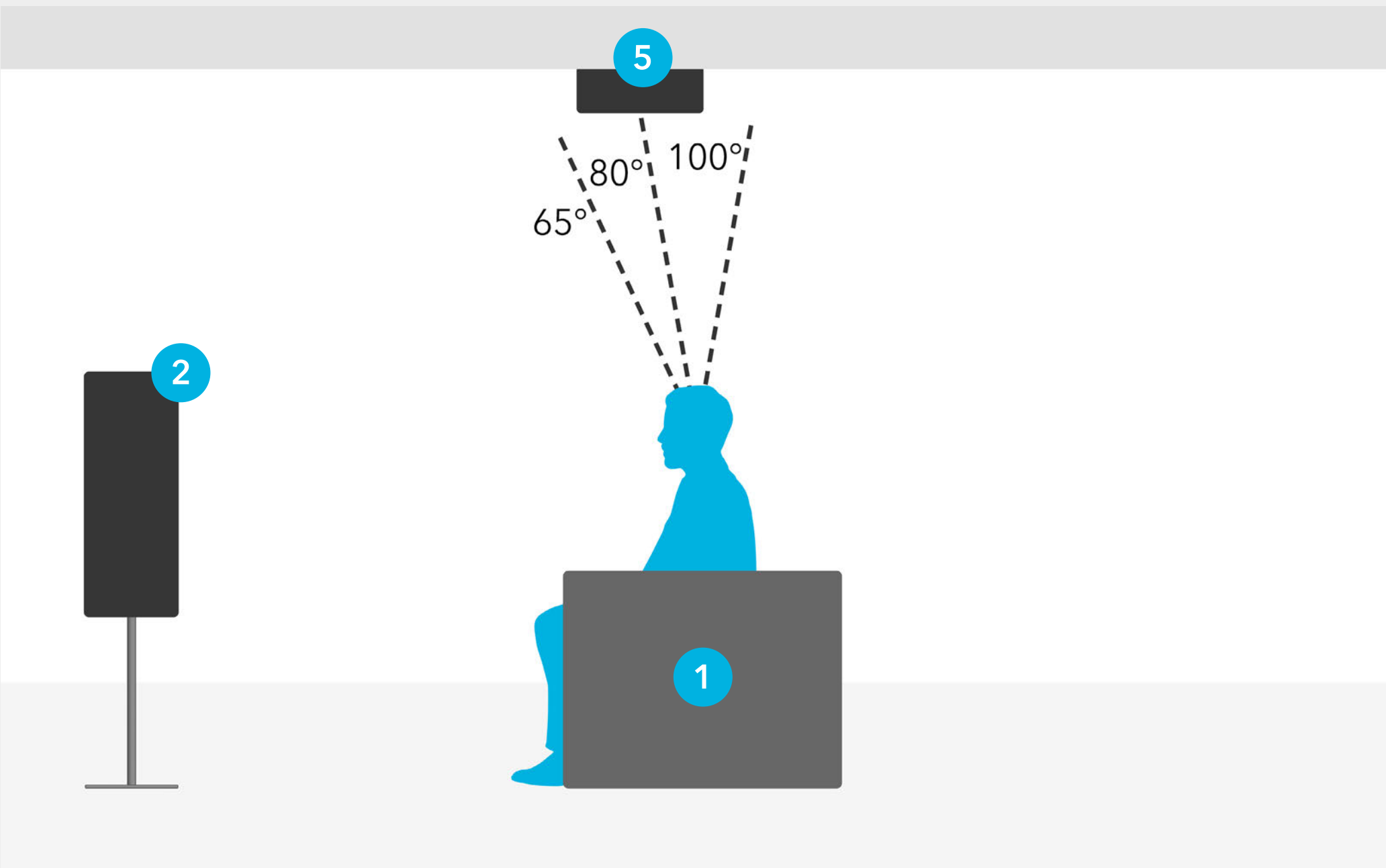
OVERHEAD SPEAKER PLACEMENT DETAIL FOR 3.1.2 SETUP
