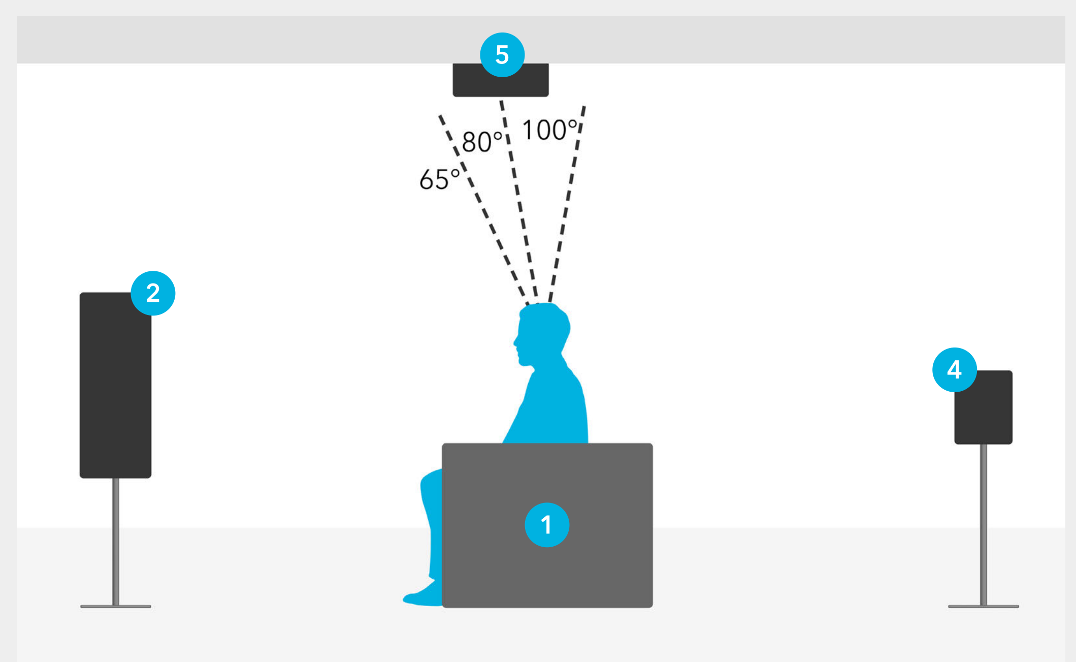
OVERHEAD SPEAKER PLACEMENT DETAIL FOR 4.1.2 SETUP
