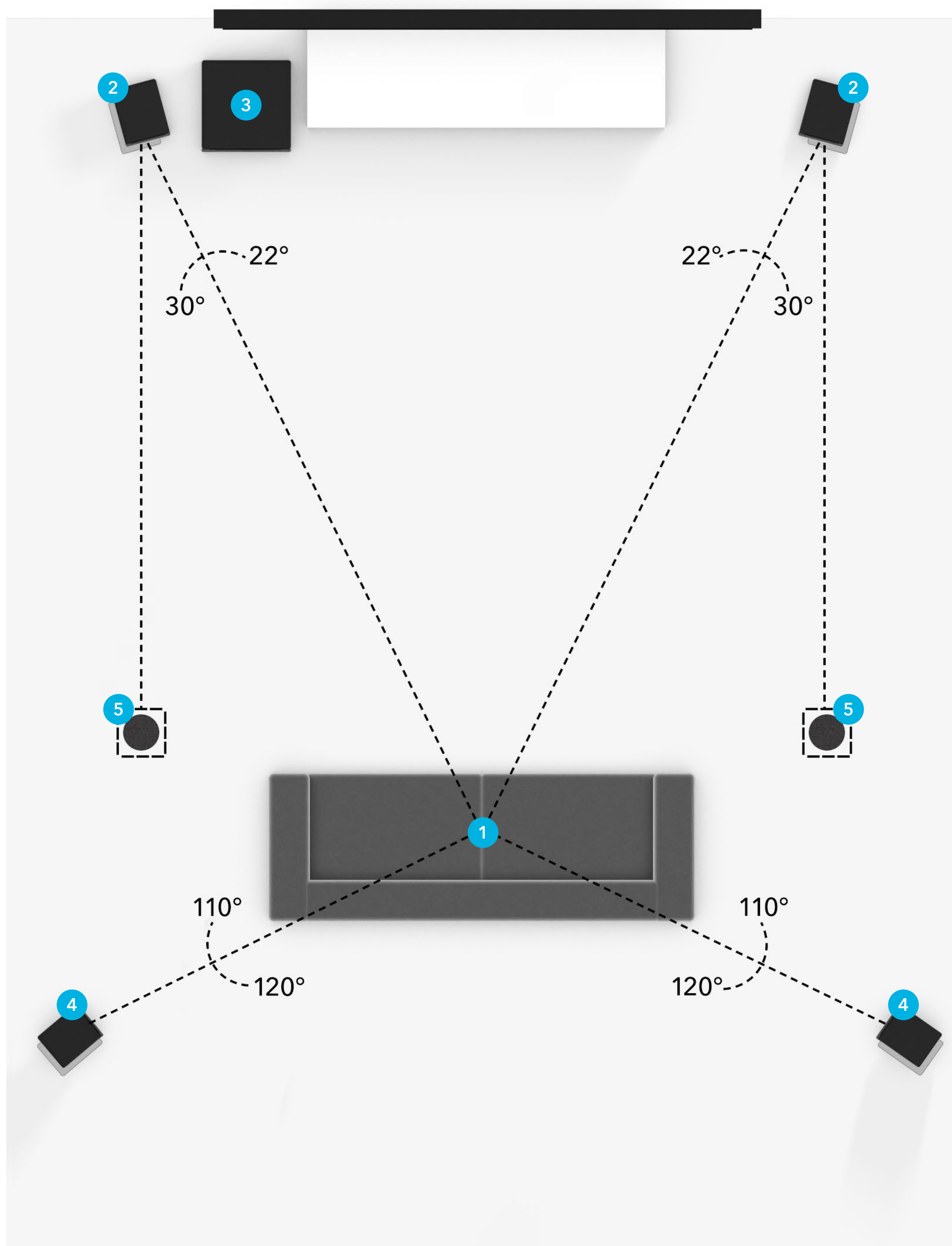
SPEAKER PLACEMENT FOR 4.1.2 SETUP
