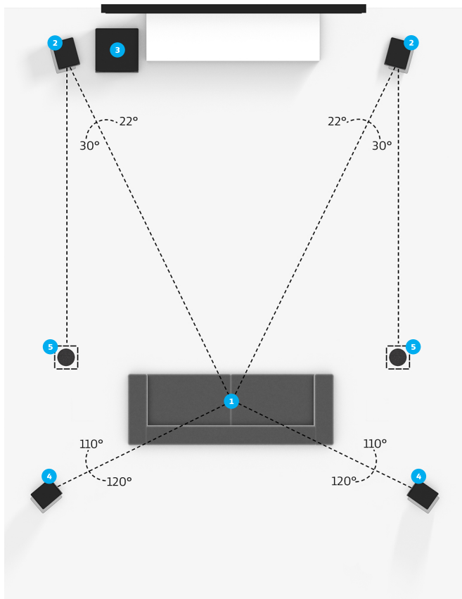
Speaker placement for 4.1.2 setup
