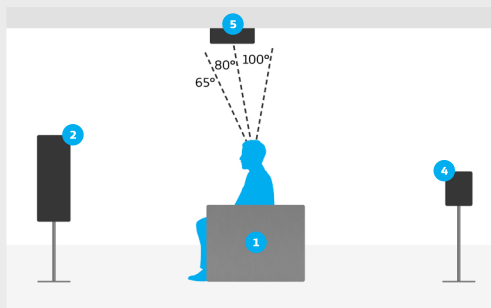
Overhead speaker placement detail for 4.1.2 setup
