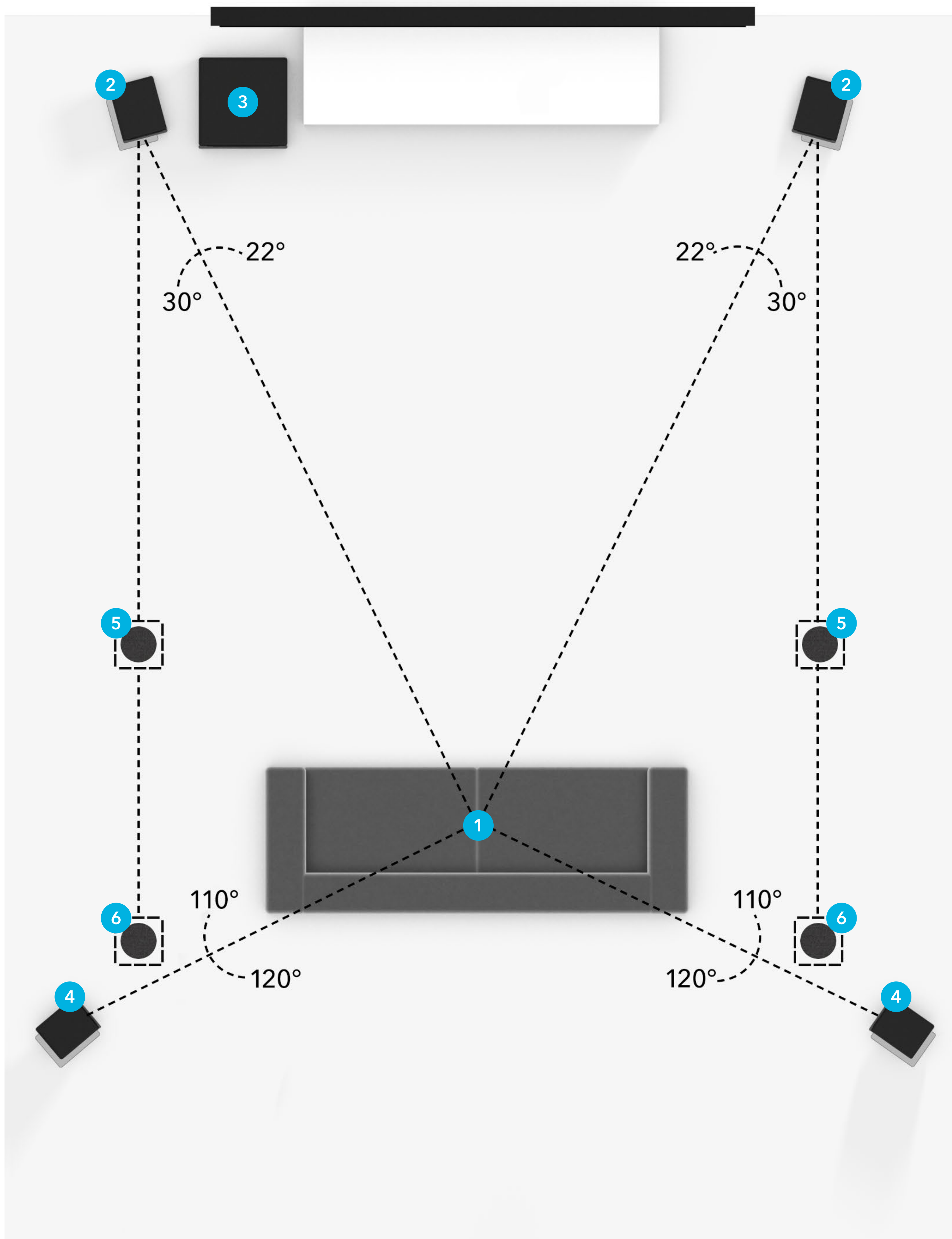
SPEAKER PLACEMENT FOR 4.1.4 SETUP
