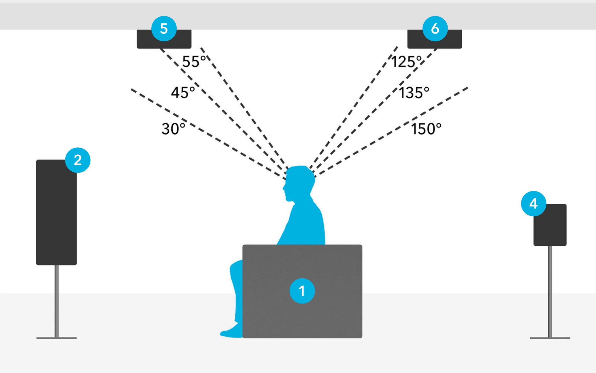
OVERHEAD SPEAKER PLACEMENT DETAIL FOR 4.1.4 SETUP
