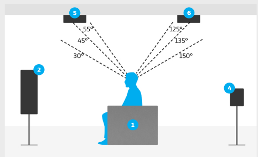
Overhead speaker placement detail for 4.1.4 setup
