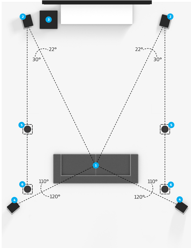
Speaker placement for 4.1.4 setup
