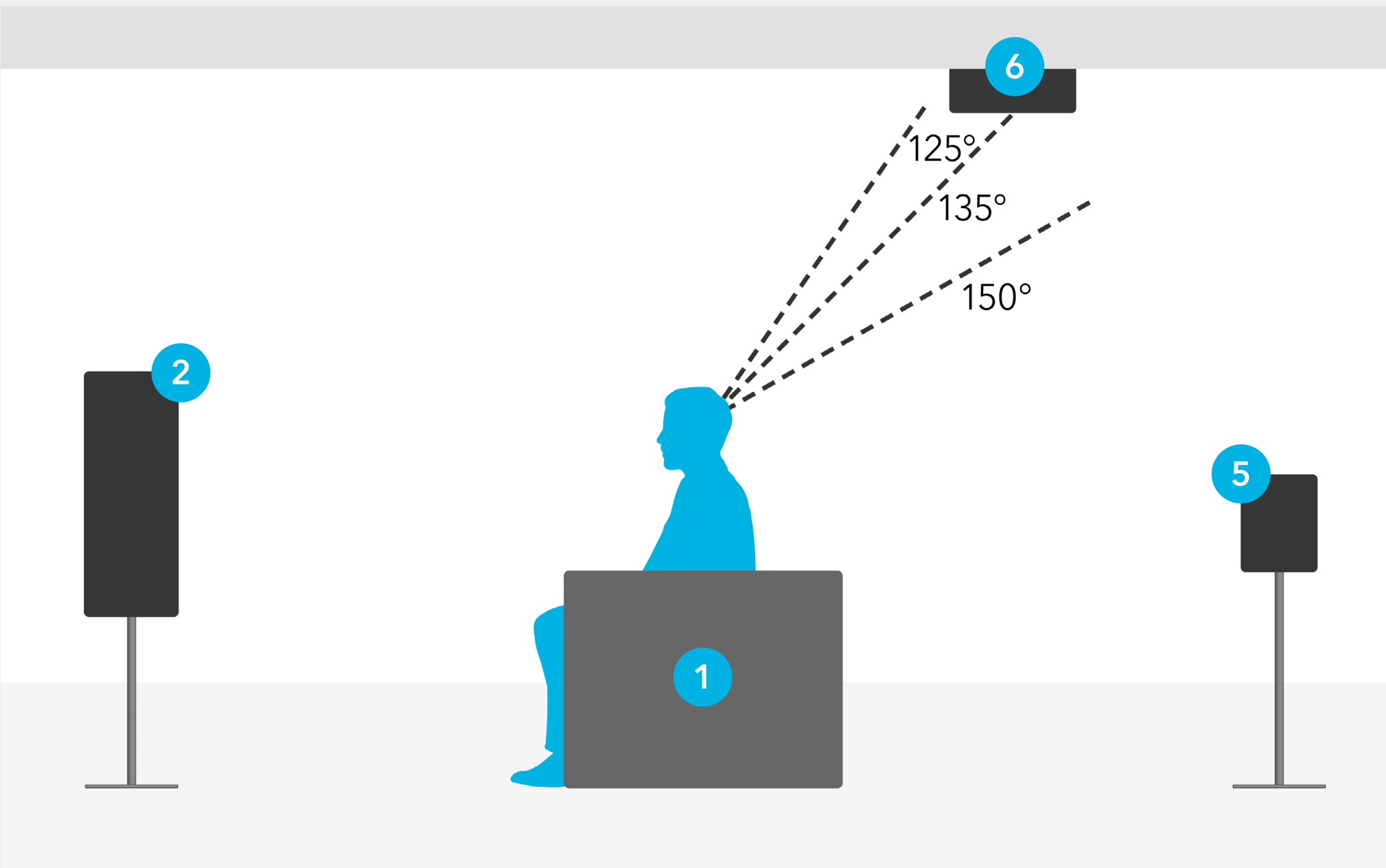
OVERHEAD SPEAKER PLACEMENT DETAIL FOR 5.1.4 HYBRID SETUP
