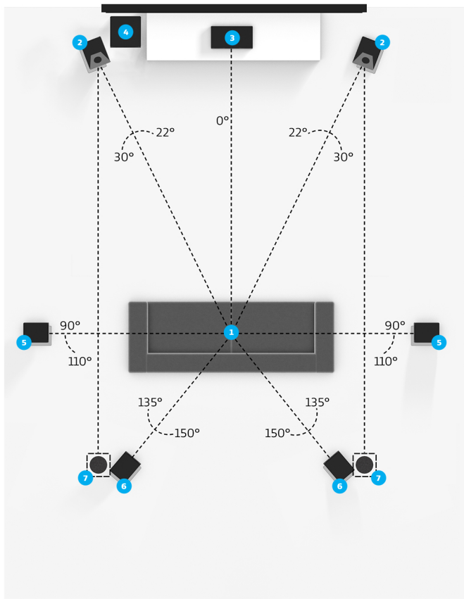
Speaker placement for 7.1.4 hybrid setup
