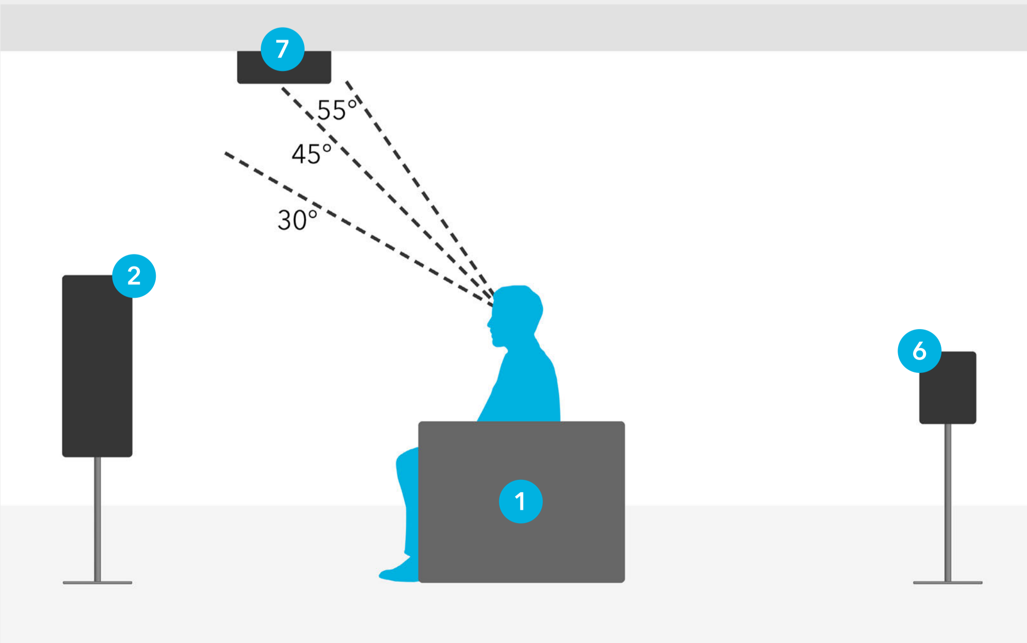
OVERHEAD SPEAKER PLACEMENT DETAIL FOR 7.1.4 HYBRID SETUP
