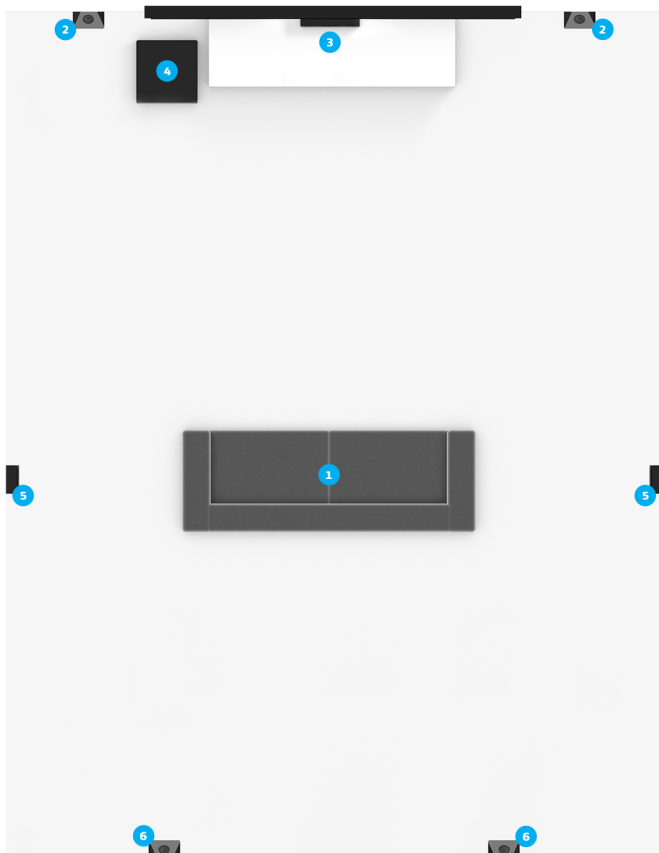
Speaker placement for 7.1.4 setup
