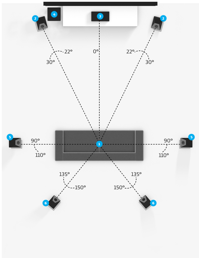
Speaker placement for 7.1.6 setup
