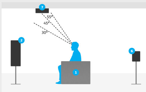
Overhead speaker placement detail for 7.1.6 hybrid setup
