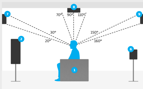
Overhead speaker placement detail for 7.1.6 setup
