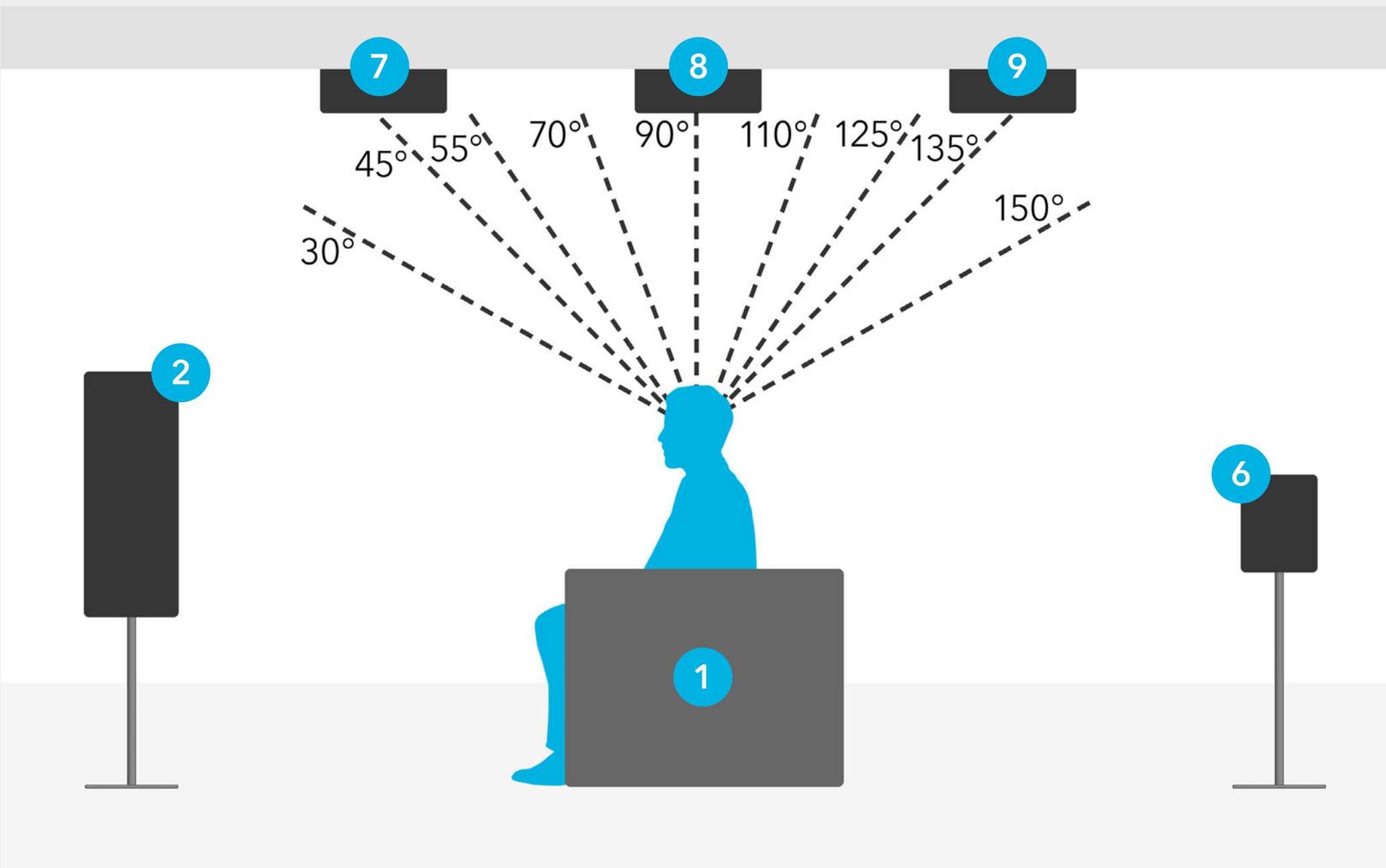
OVERHEAD SPEAKER PLACEMENT DETAIL FOR 7.1.6 SETUP
