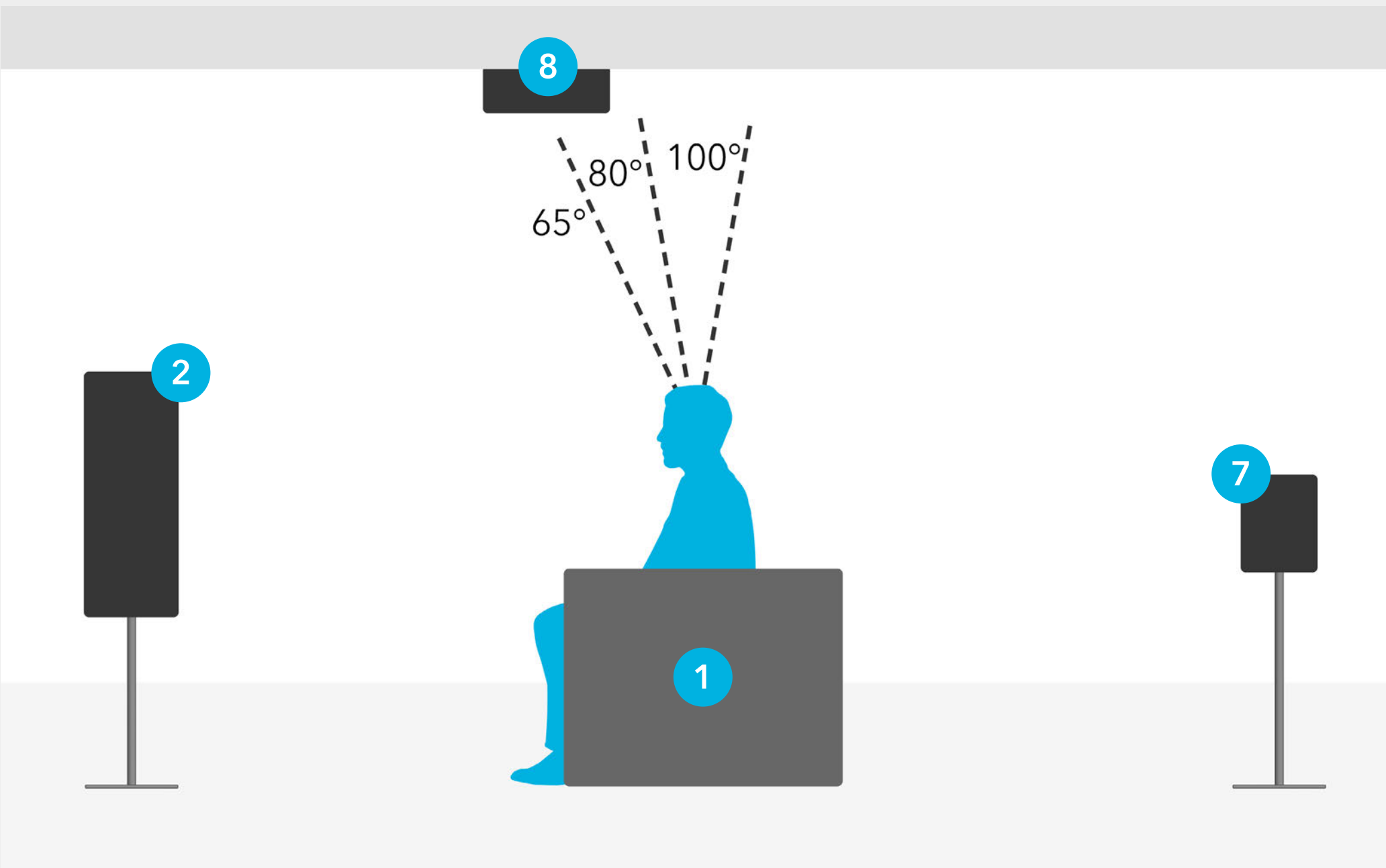
OVERHEAD SPEAKER PLACEMENT DETAIL FOR 9.1.2 SETUP
