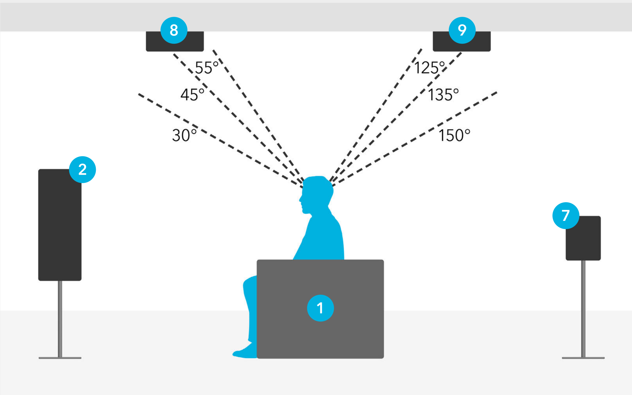
OVERHEAD SPEAKER PLACEMENT DETAIL FOR 9.1.4 SETUP
