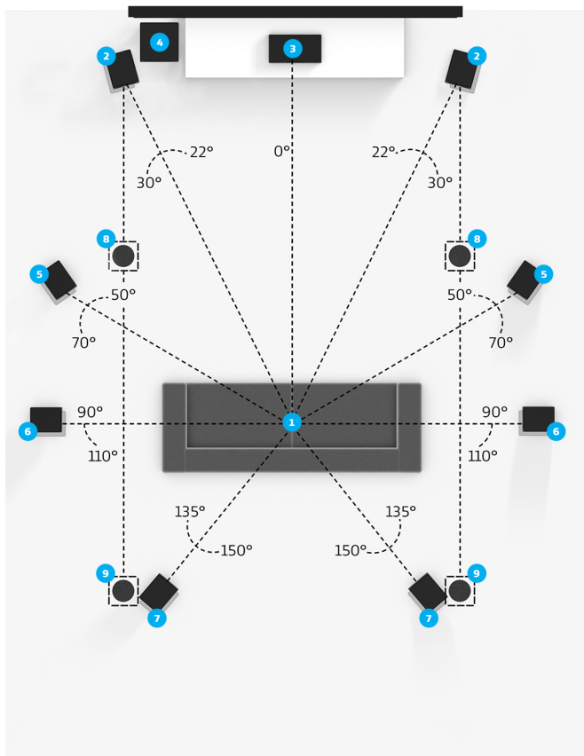
Speaker placement for 9.1.4 setup
