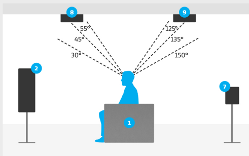
Overhead speaker placement detail for 9.1.4 setup
