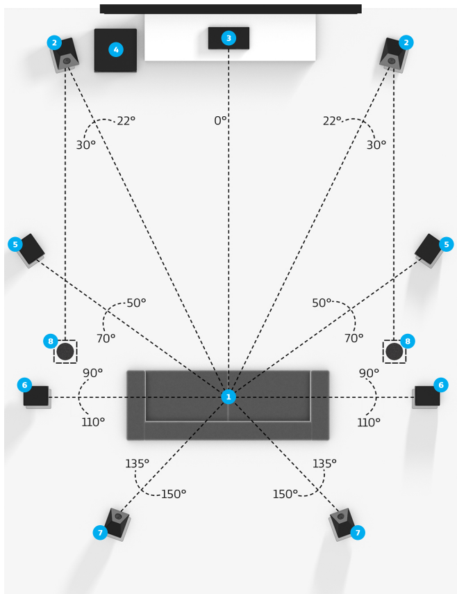
Speaker placement for 9.1.6 setup
