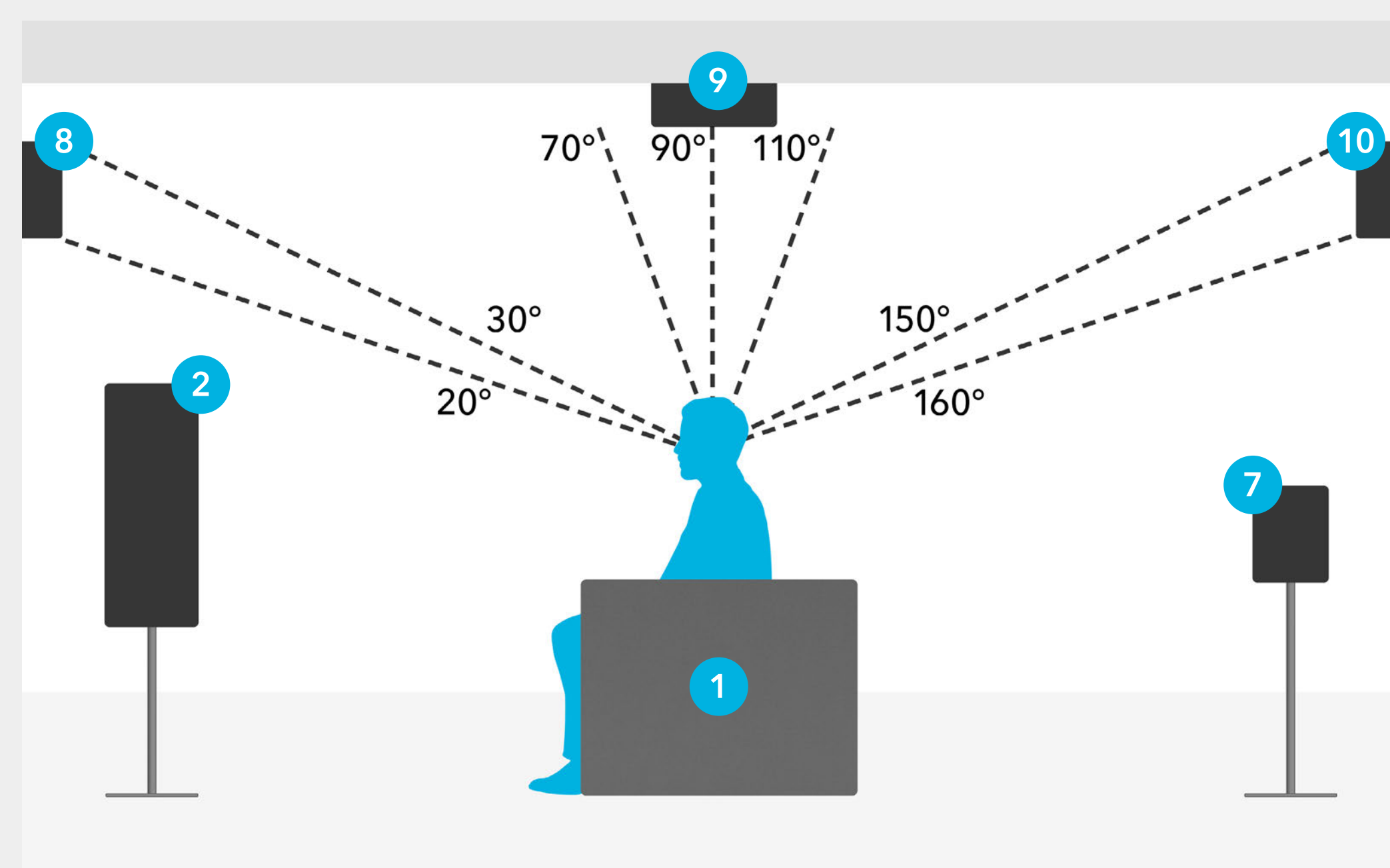
OVERHEAD SPEAKER PLACEMENT DETAIL FOR 9.1.6 SETUP
