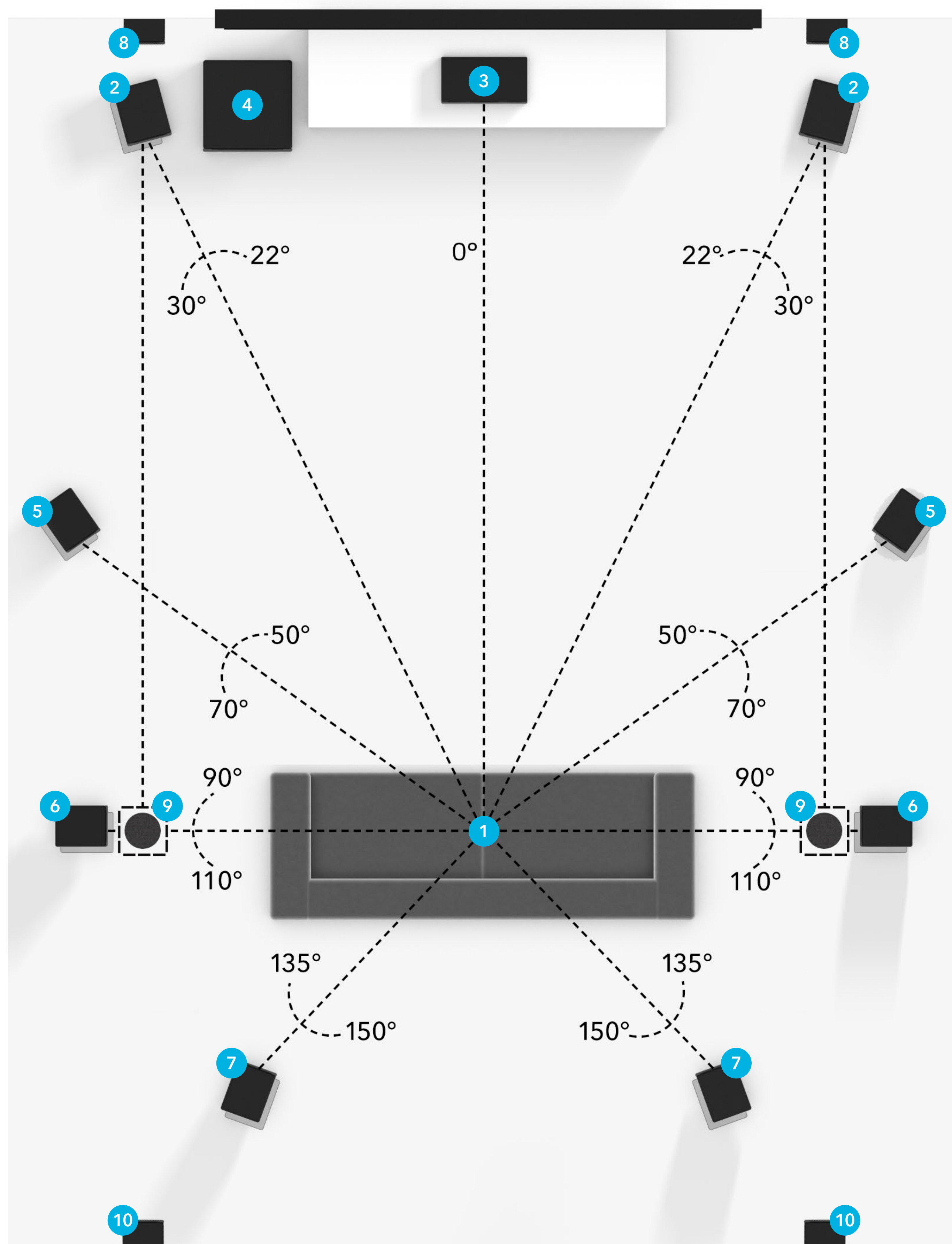
SPEAKER PLACEMENT FOR 9.1.6 SETUP
