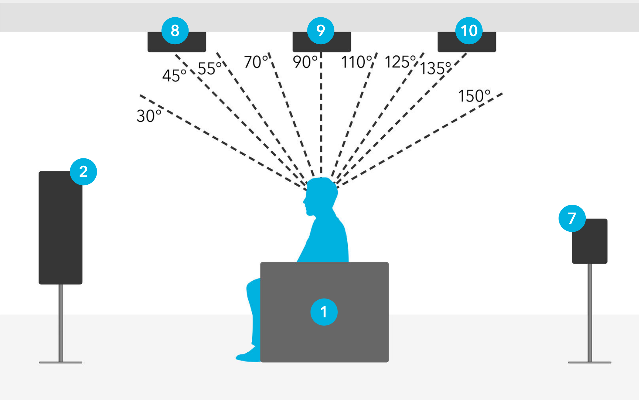
OVERHEAD SPEAKER PLACEMENT DETAIL FOR 9.1.6 SETUP
