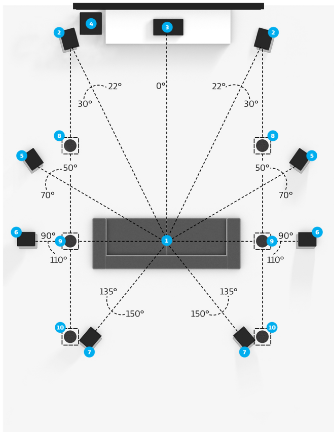
Speaker placement for 9.1.6 setup
