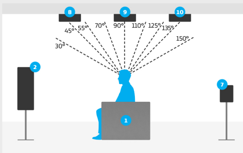
Overhead speaker placement detail for 9.1.6 setup
